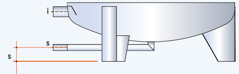
Detail of the total drain pipe only for the 2000 litres model
